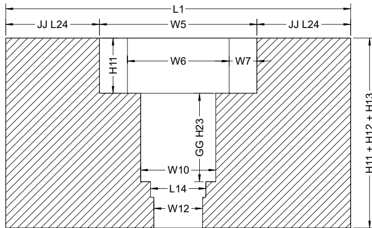
Section H-H
