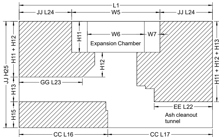
Section J-J
